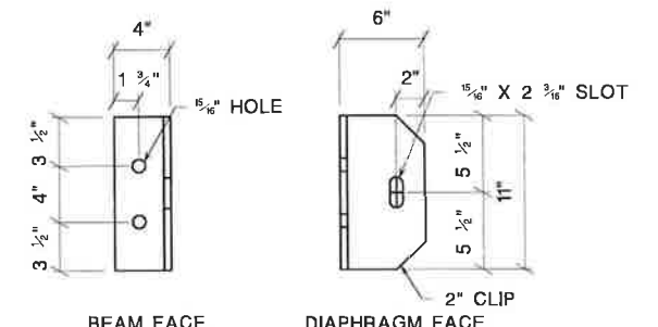
CL11B INTERIOR BEAM ONLY
