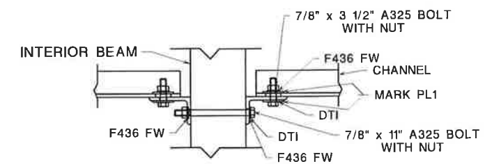
INTERIOR SQUARE CONNECTION DETAIL
