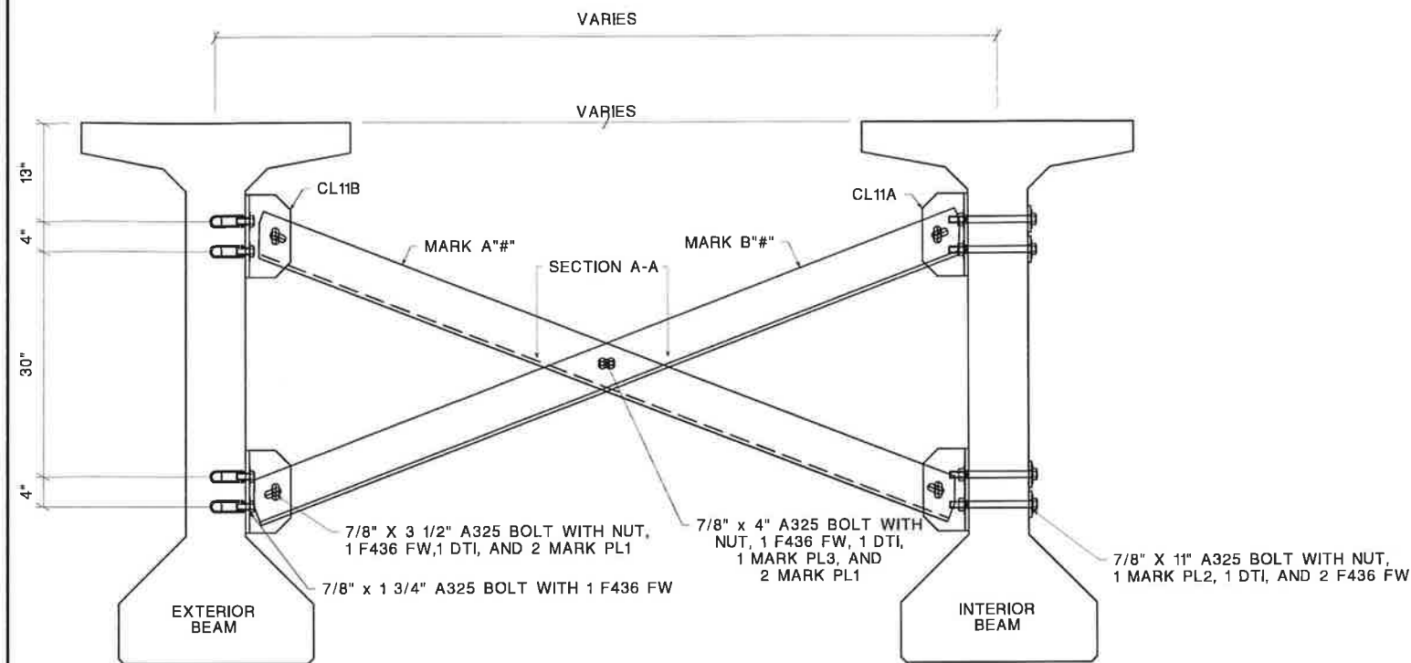
TYPICAL SKEW SECTION
