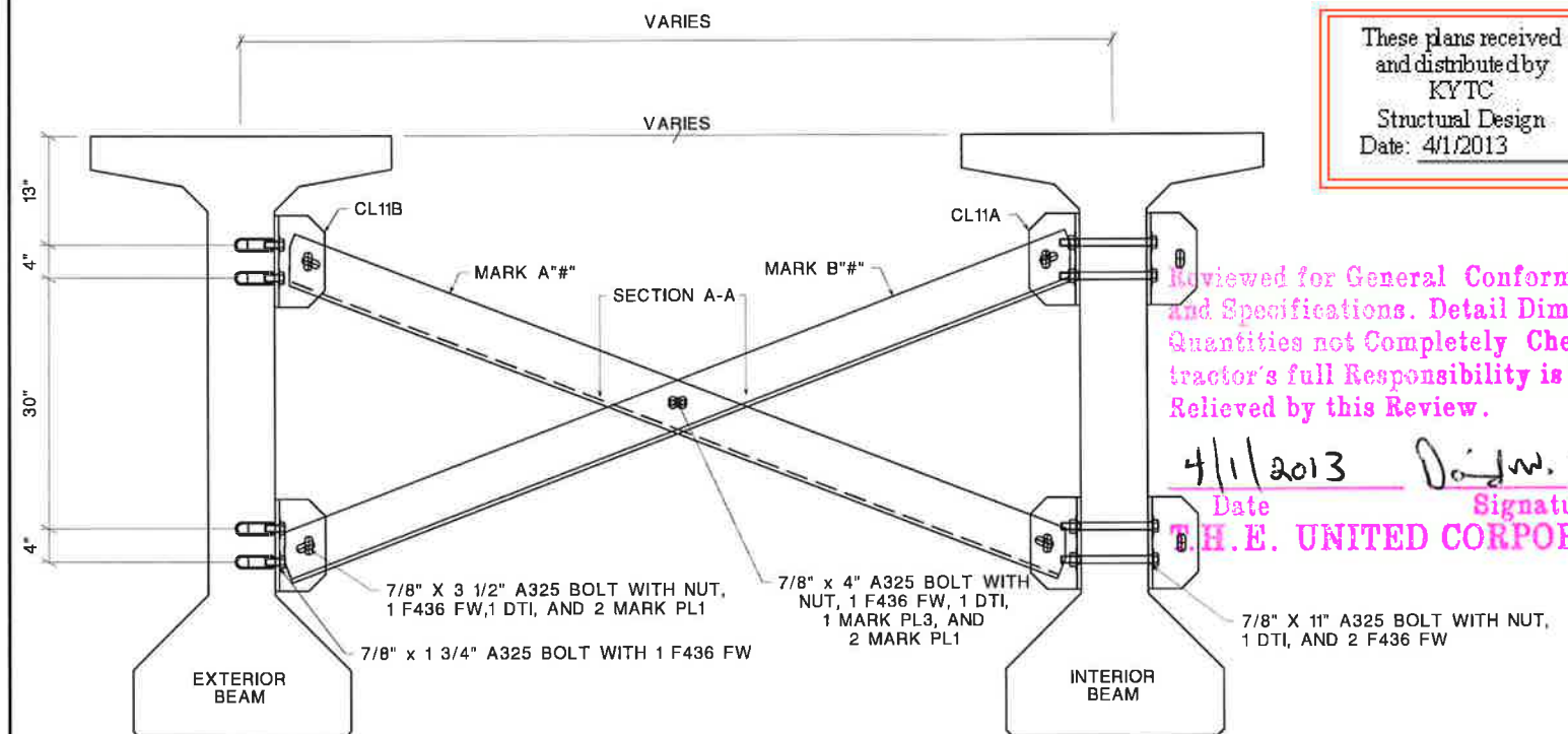
TYPICAL SQUARE SECTION
