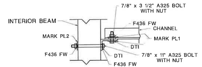
INTERIOR SKEW CONNECTION DETAIL
