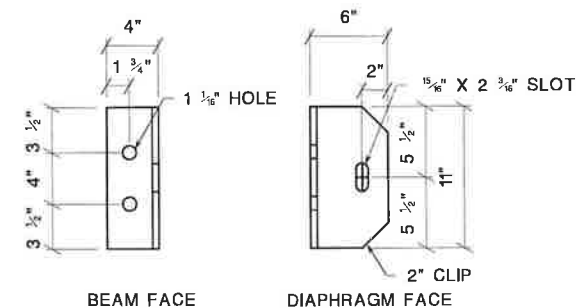
CL11A INTERIOR BEAM ONLY
